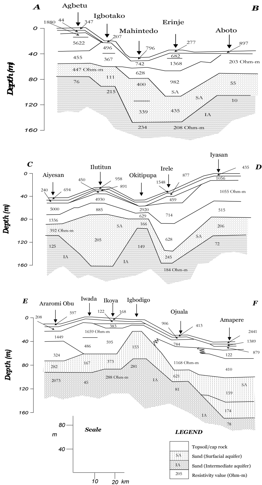
Figure 4: Goelectric Section along North-South (AB), West-East(CD), and Northwest-Southeast Directions in the Area.
