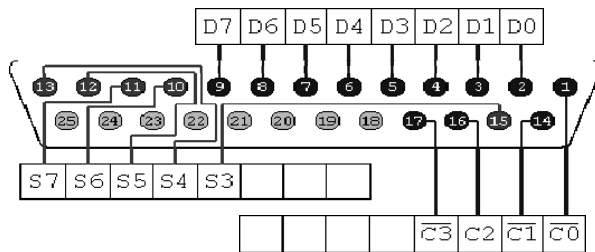
Figure 1: DB25 Connector for Parallel Port.
