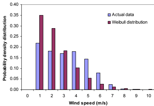
Figure 5: Comparison of Actual Wind Speed Probability Distribution for the Whole Year with Weibull Approximations.
