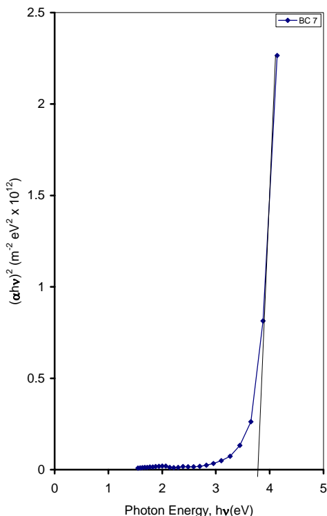
Figure 13: Plot of (\alpha hv)^2 against hv for BiClO Sample .
