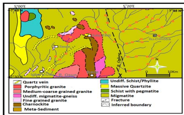
Figure 2: Geological Map of Ado Ekiti (after Talabi and Tijani, 2012).
