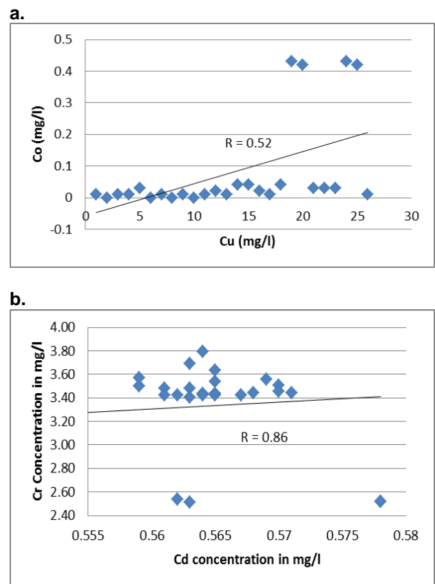
Figure 6: Scatter Plots Showing Variations among a) Co vs Cu b) Cr vs Cd.
