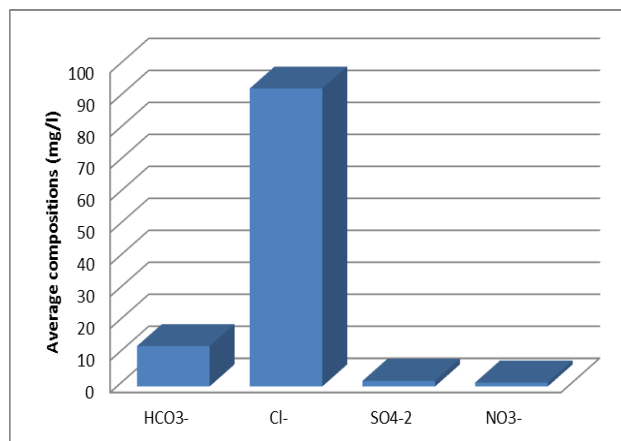
Figure 5: Comparison among the Mean Values of Anions.
