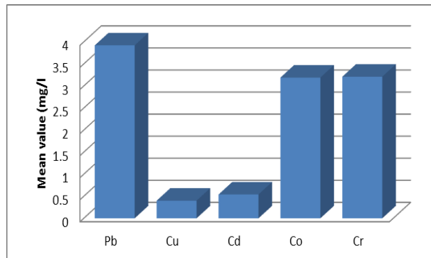
Figure 4: Comparison among the Mean Values of Trace Elements.
