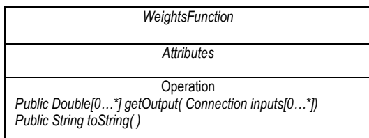
Figure 10: UML Class Diagram for the WeightFunction.
