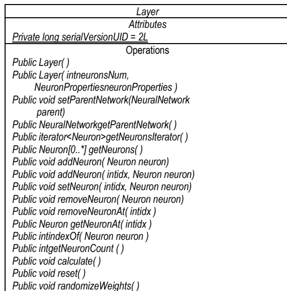
Figure 1: UML Class Diagram for the Layer.
