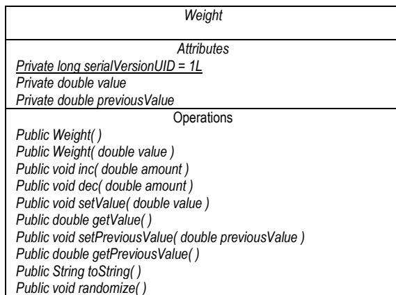
Figure 4: UML Class Diagram for the Weight.
