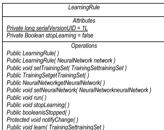
Figure 5: UML Class Diagram for the LearningRule.
