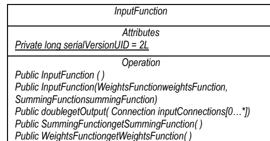
Figure 7: UML Class Diagram for the InputFunction.
