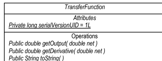
Figure 8: UML Class Diagram for the TransferFunction.
