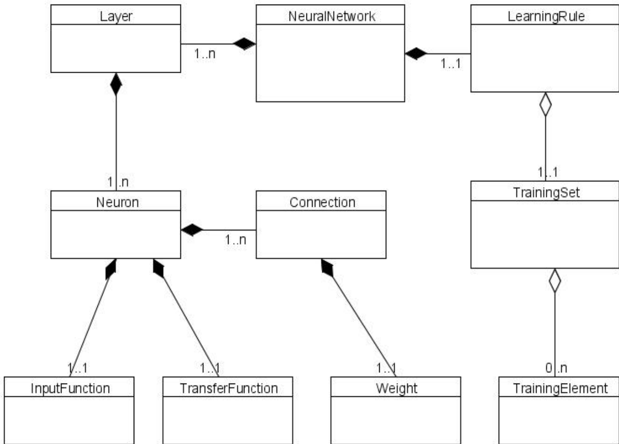
Figure 14: the architectural design of the system
