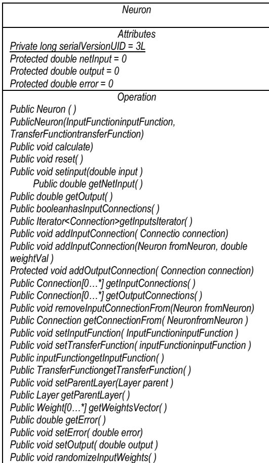
Figure 9: UML Class Diagram for the Neuron.
