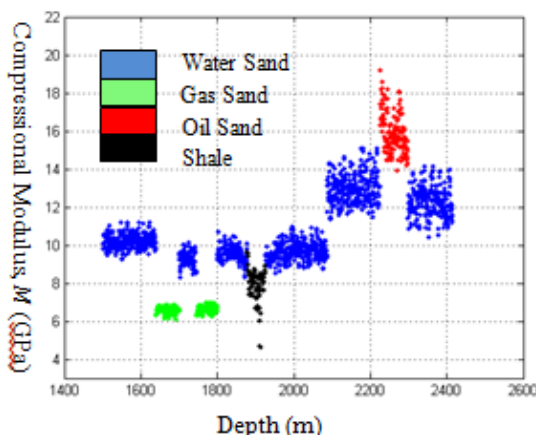
Figure 4: Estimated Compressional Modulus versus Depth in the Logged Interval. The plot shows the sensitivity of compressional modulus to different pore fluids and lithologies
