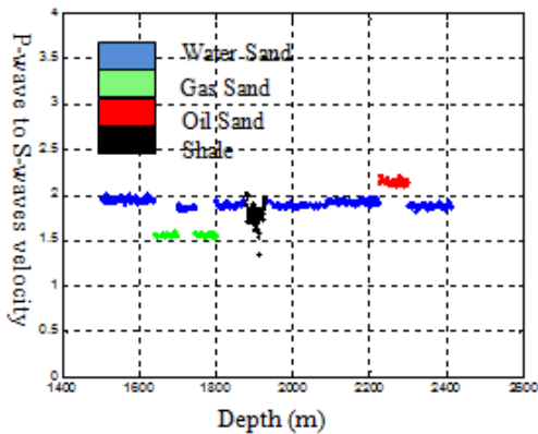
Figure 8: The Estimated P-wave to S-waves Velocity Ratio versus Depth in the Logged Interval. The velocity ratio discriminates between pore fluids. It is also sensitive to the change of lithology.
