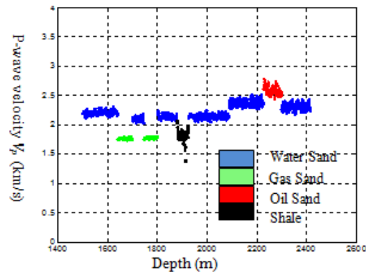
Figure 6: The Estimated P-Wave Velocity versus Depth in the Logged Interval. P-wave velocity is sensitive to change of pore fluid and lithology.
