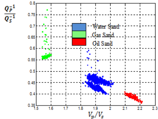
Figure 11: Cross Plot of the Ratio of the Inverse Quality Factor ( Q_P^{-1}/Q_S^{-1} ) and the Velocity Ratio ( V_P/V_S ). Colour index is shown in the legend.
