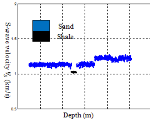
Figure 7: Estimated S-Wave Velocity versus Depth in the Logged Interval. S-wave velocity is not sensitive to change of pore fluid, but sensitive to change of lithology
