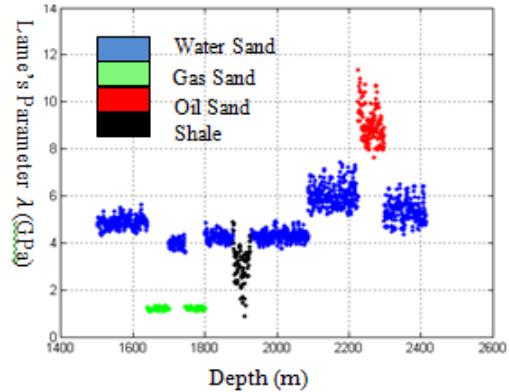
Figure 5: Estimated Lamé's First Parameter versus Depth. The plot shows the sensitivity of Lamé's first parameter to change of pore fluid.
