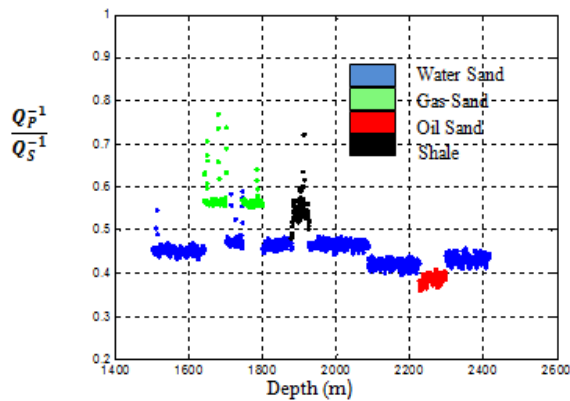
Figure 10: The Estimated Inverse Quality Factor Ratio, Q_P^{-1}/Q_S^{-1} Plotted with Depth. Colour index is shown in the legend. (V_P/V_S)
