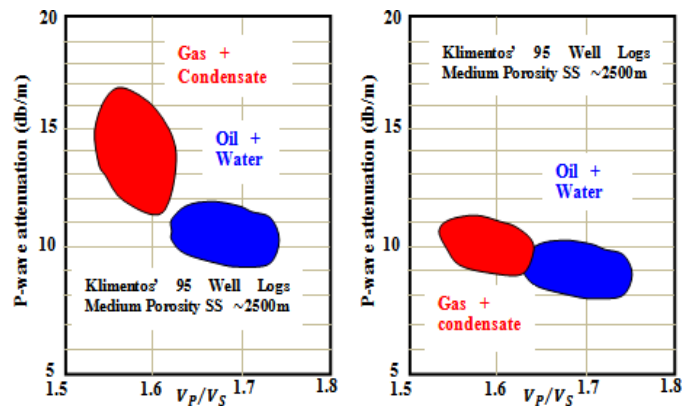
Figure 12: P-wave and S-wave Attenuation Calculated from Full-Waveform Sonic and Dipole Log Data in Medium-Porosity Sandstone with Oil, Water, Gas and Condensate by Klimentos (1995). Adopted from Mavko et al. (2005).
