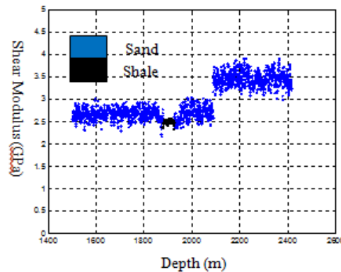
Figure 3: The Estimated Shear Modulus versus Depth. Shear modulus is not sensitive to pore fluid but sensitive to change of lithology (sand – shale – sand) due to the changes in mineral matrix.
