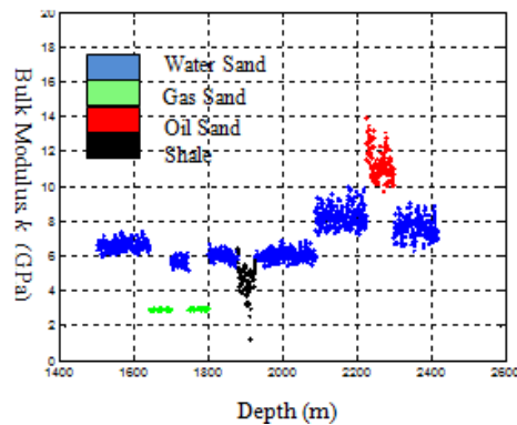
Figure 2: The Estimated Bulk Modulus versus Depth- showing sensitivity of the bulk modulus to different fluids in the rocks in logged interval. Bulk modulus is also sensitive to changes in lithology. It registers different values for water saturated sand and water saturated shale.
