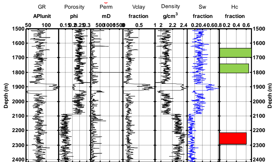
Figure 1: Well Log Curves: shown from left to right are: Gamma ray log, Porosity log, Permeability log, Clay volume log, Bulk density log, Water saturation log and Hydrocarbon saturation log. The three logs are from Gullfaks Well A-10. Others log curves are estimated using some quantitative models. In Hydrocarbon log, green is gas and red is oil. See the electronic version for colour codes.
