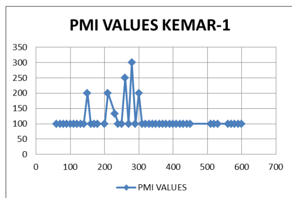
Figure 7: Palynomorph Marine Index (PMI) Chart of Kamar-1 Well.
