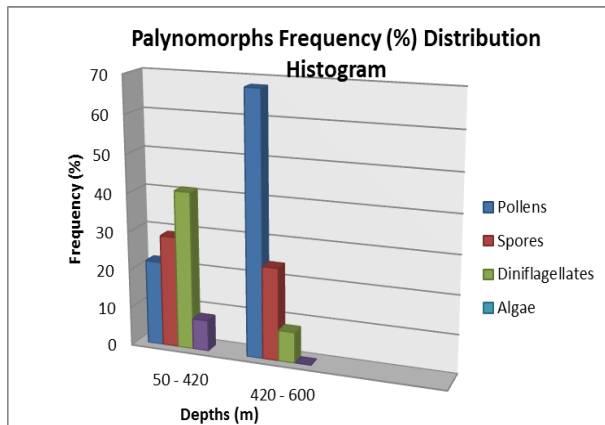
Figure 5: Histogram of Frequency (%) Palynomorphs Distribution (Kemar-1).
