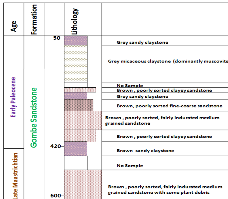
Figure 2: Lithological Section and Description of Interval 50-600m in the Kemar – 1 Well.
