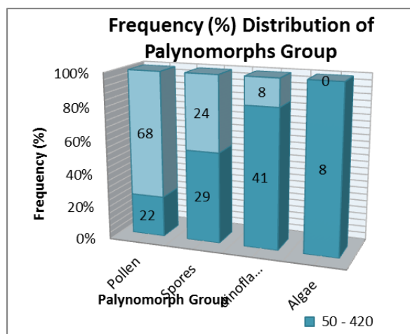
Figure 4: Frequency Distribution Plot of Palynomorphs in Kamar-1 Well.
