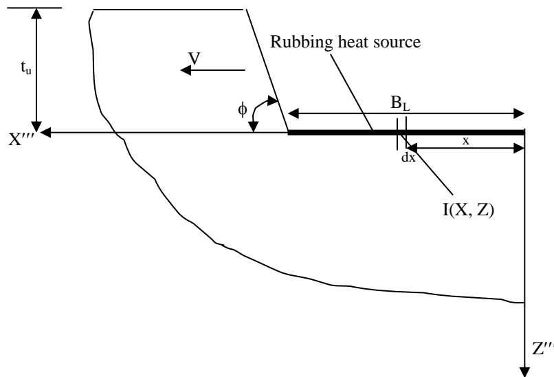
Figure 8: Thermal Modeling of Rubbing Heat Source on the Workpiece Side (Trigger et al., 1957). The temperature rise on the workpiece was given as, Ceretti et al (1996):
