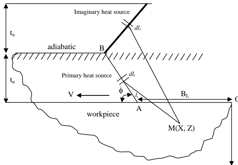
Figure 6: Thermal Modeling of Primary Heat Source on the Workpiece Side (adapted from Boothroyd, 1963).
