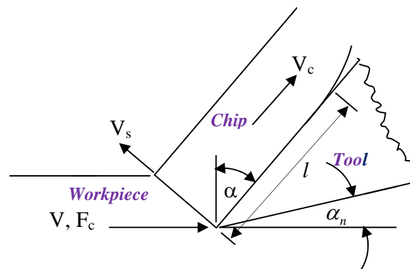
Figure 1: Continuous Chip Formation in Orthogonal Cutting Process.
