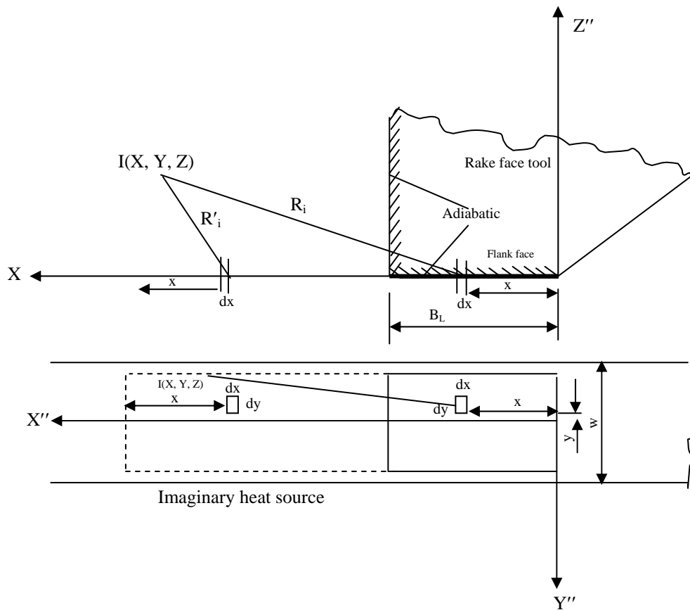
Figure 7: Thermal Modeling of Rubbing Heat Source on the Tool Rake and Flank Faces for a Blunt Tool (modified from Murarka et al., 1981).
