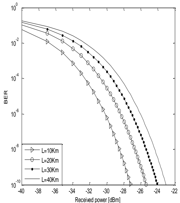
Figure 5: Plot of BER versus Received Power for Different Fiber Lengths when Chip Rate=100 Gchip/s, Pulse Linear Chirp C=1 , and 10 Number of Simultaneous User.
