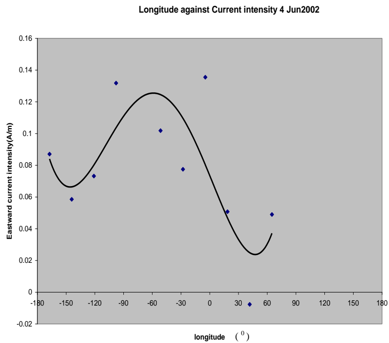
Figure 5: Fairly Systematic Longitudinal Variation on 4 June, 2002.
