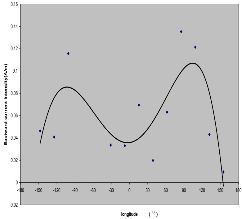
Figure 6: Unsystematic Longitudinal Variation on 14 June, 2002.
