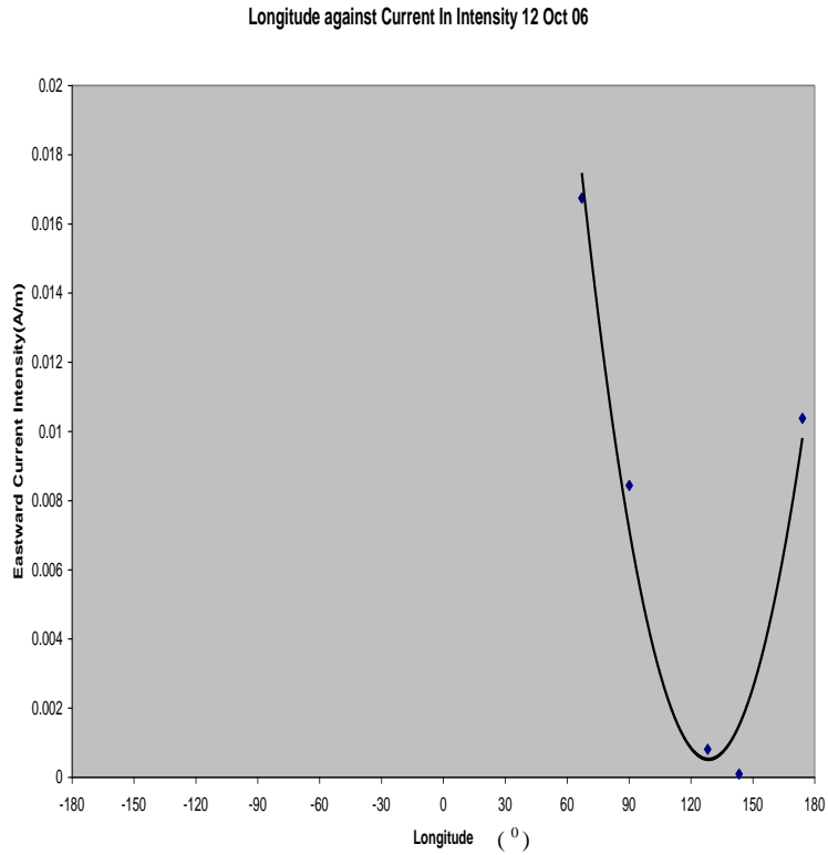
Figure 14: Systematic Longitudinal Variation on 12 October, 2006.
