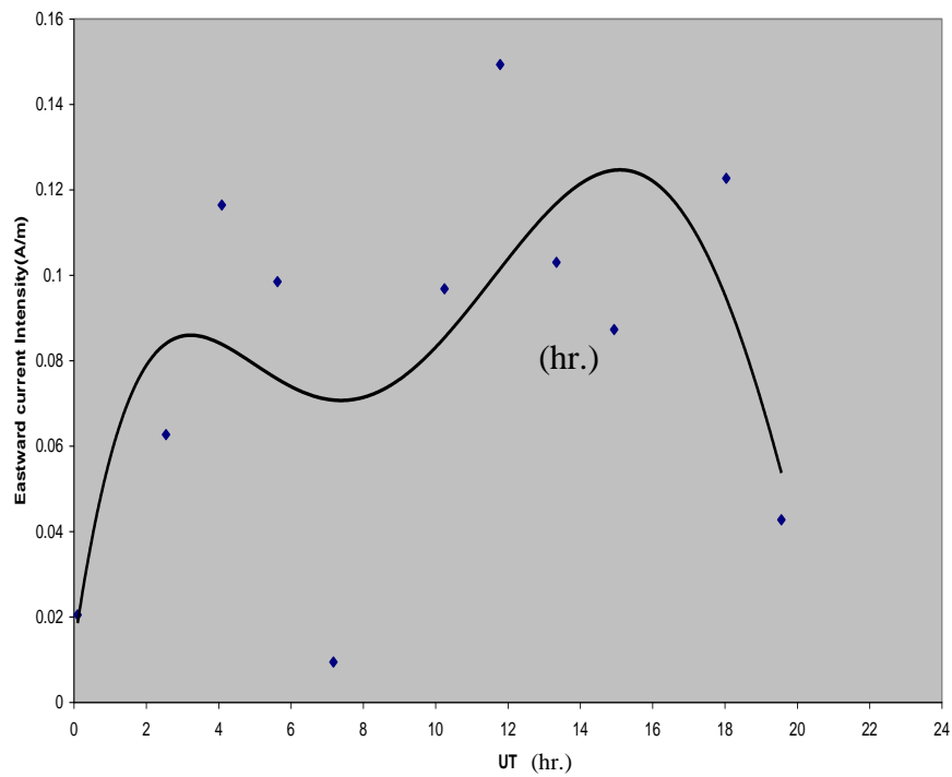
Figure 20: Unsystematic UT variation on 6 June 2002.
