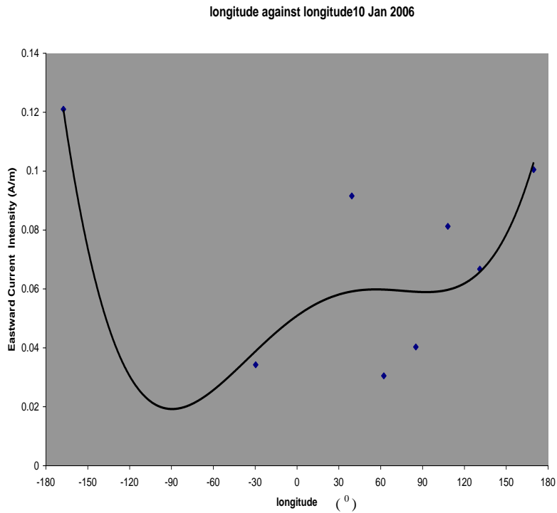
Figure 10: Unsystematic Variation of the EEJ Intensity on 10 January, 2006.
