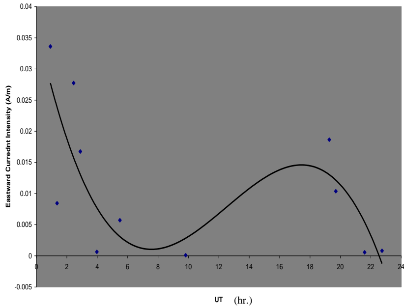
Figure 25: Unsystematic UT Variation on 15 October 2006.
