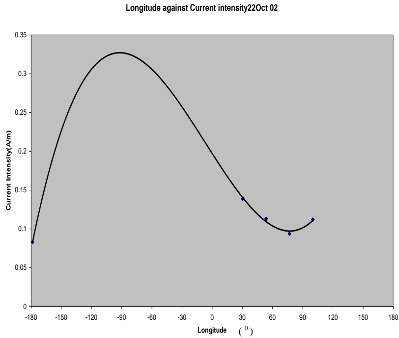
Figure 8: Systematic Variation of the EEJ Intensity on 22 October, 2002.
