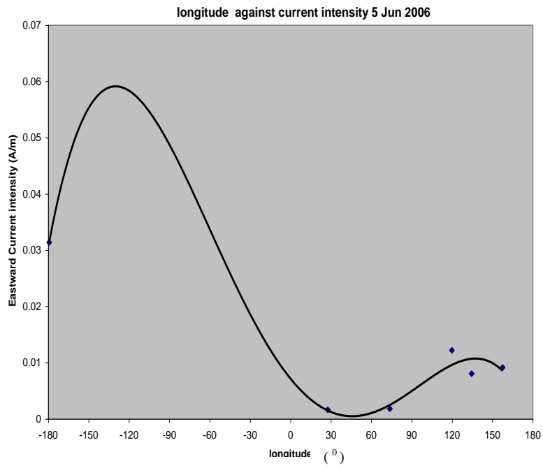
Figure 12: Systematic Longitudinal Variation of the EEJ Intensity on 5 June 2006.
