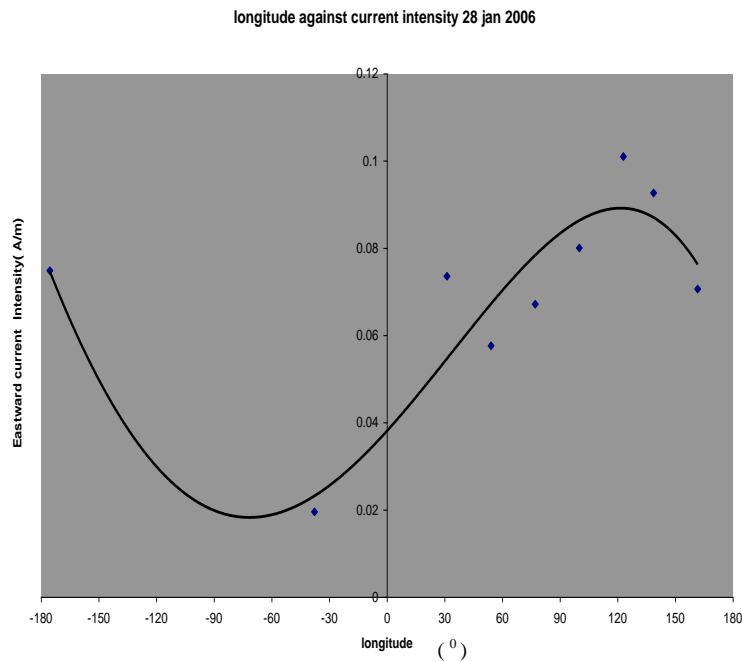
Figure 11: Fairly Systematic Variation of the EEJ Intensity on 28 January 2006.
