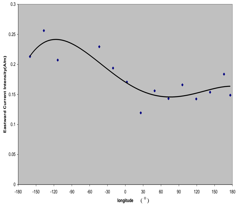
Figure 3: Systematic Longitudinal Variation on 29 January, 2002.
