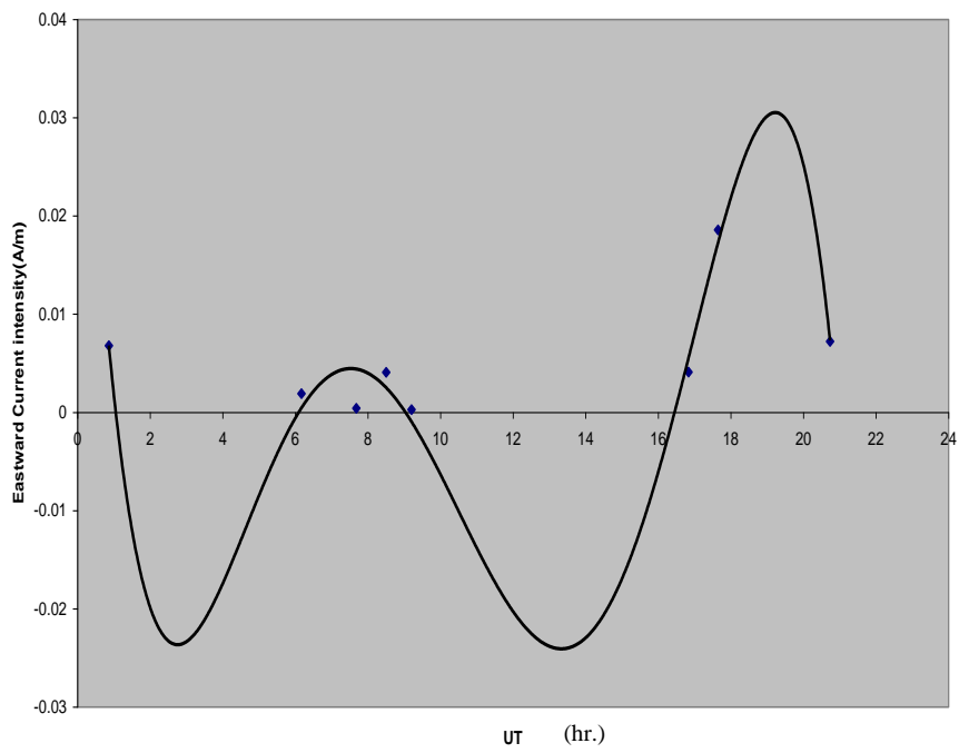
Figure 28: Unsystematic UT Variation on 19 October 2006.
