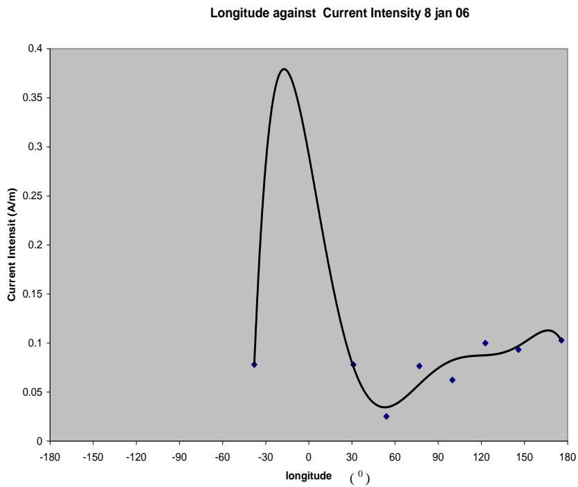
Figure 9: Systematic Variation of the EEJ Intensity on 8 January, 2006.
