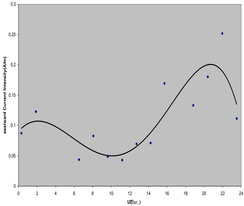
Figure 17: Fairly Systematic UT Variation on 23 January, 2002.
