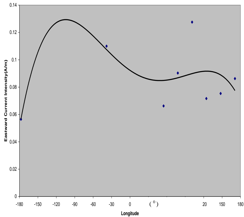
Figure 7: Fairly Systematic Longitudinal Variation on 12 October, 2002.
