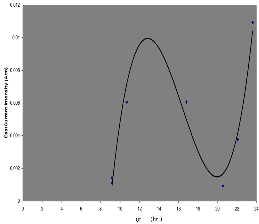
Figure 23: Systematic UT on 18 June 2006.
