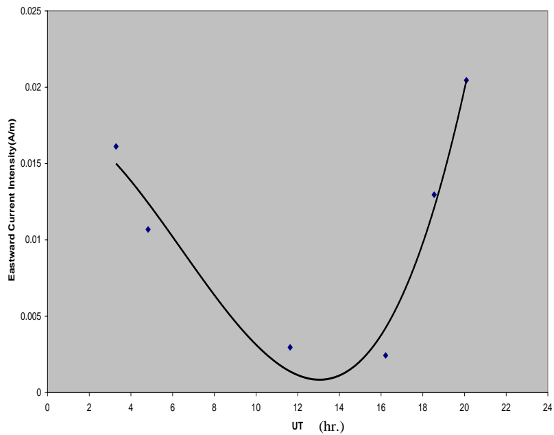
Figure 24: Systematic UT Variation on 11 June 2006.
