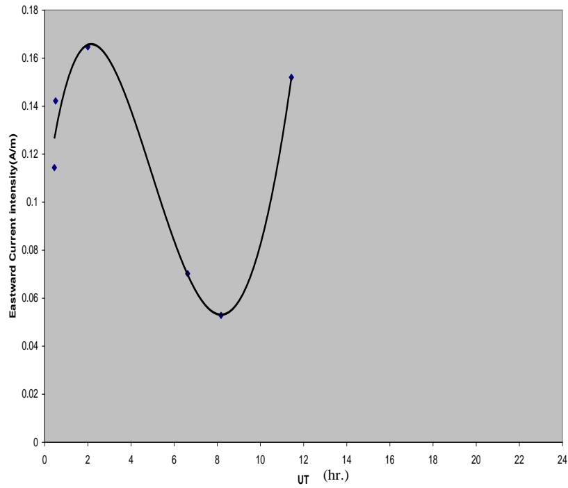
Figure 22: Systematic UT Variation on 23 October 2002.
