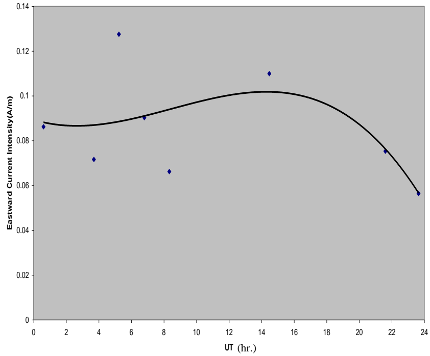
Figure 21: Unsystematic UT Variation on 12 October 2002.
