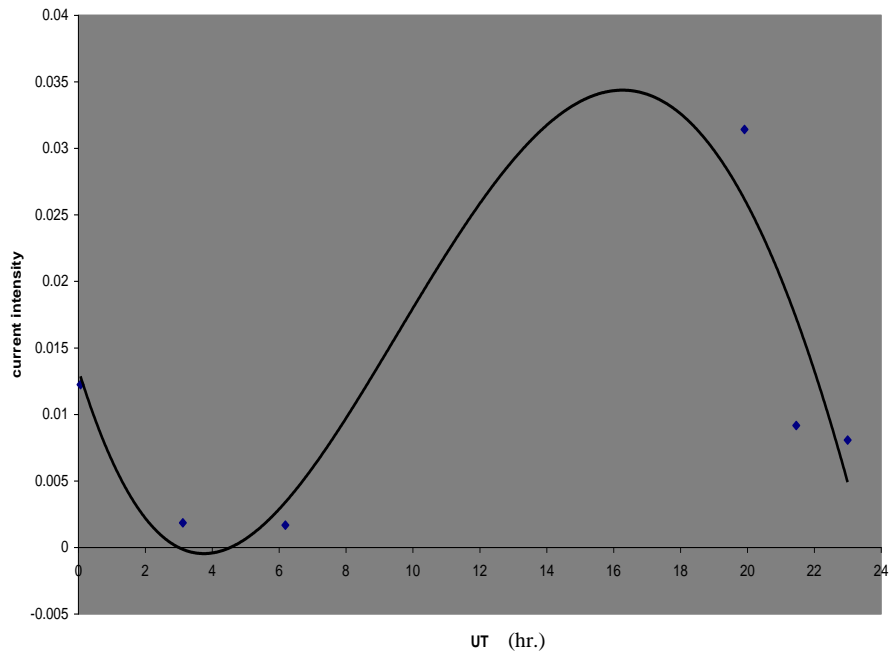
Figure 19: Systematic UT Variation on 5 June 2006.
