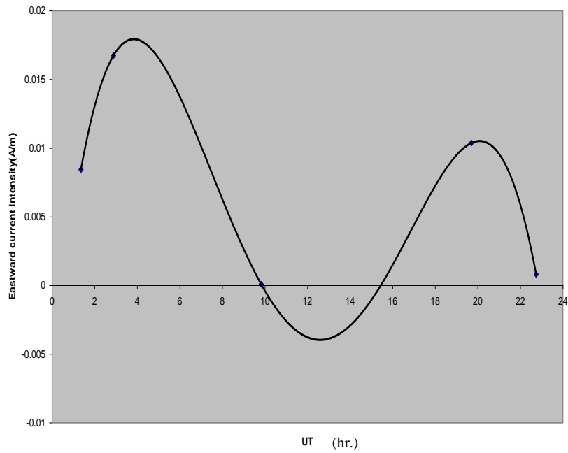
Figure 27: Unsystematic UT Variation on 12 October 2006.
