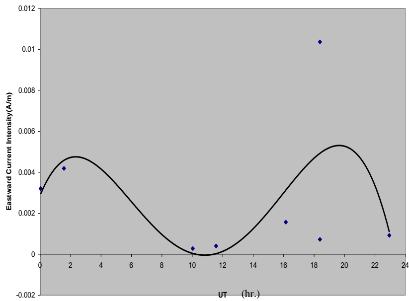
Figure 26: Unsystematic UT Variation on 20 October 2006.
