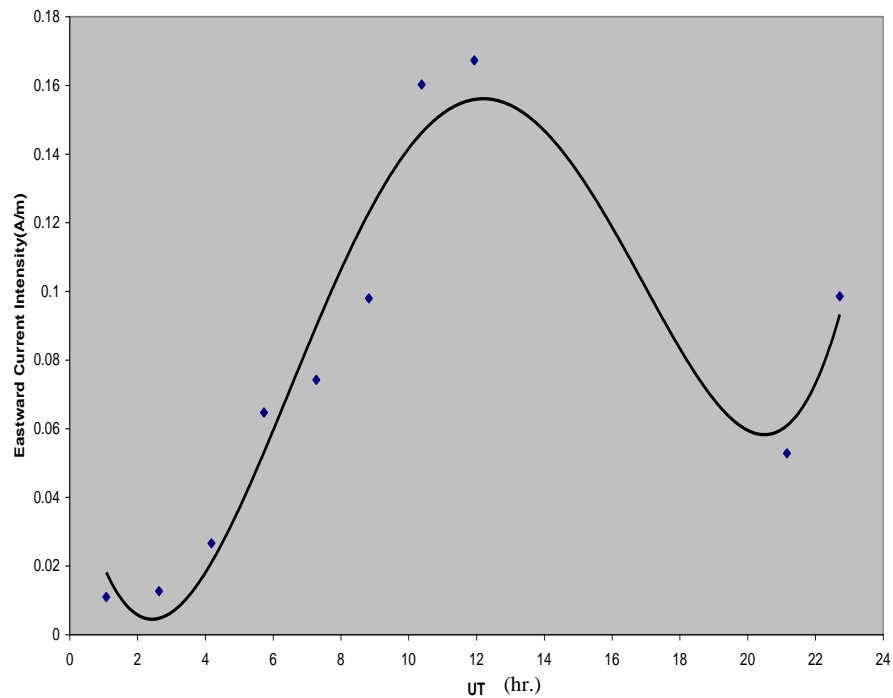
Figure 18: Systematic UT Variation on 24 January 2002.
