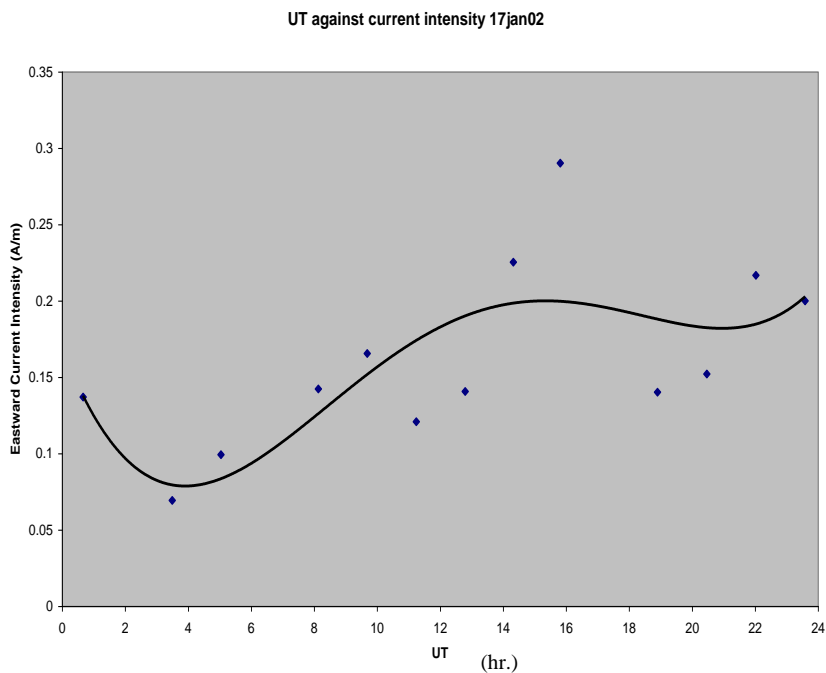
Figure 16: Fairly Systematic UT Variation on 17 January, 2002.
